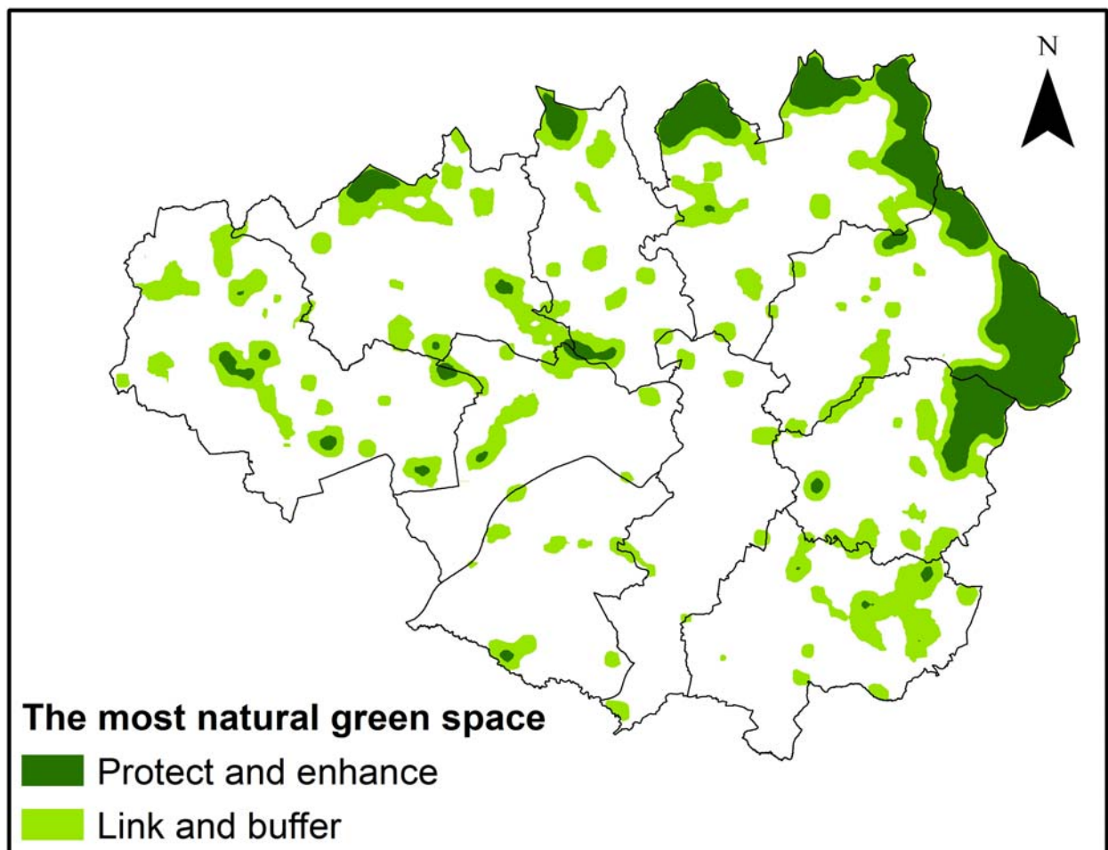
Fig 3 The Most Natural Biodiversity Opportunity Areas
